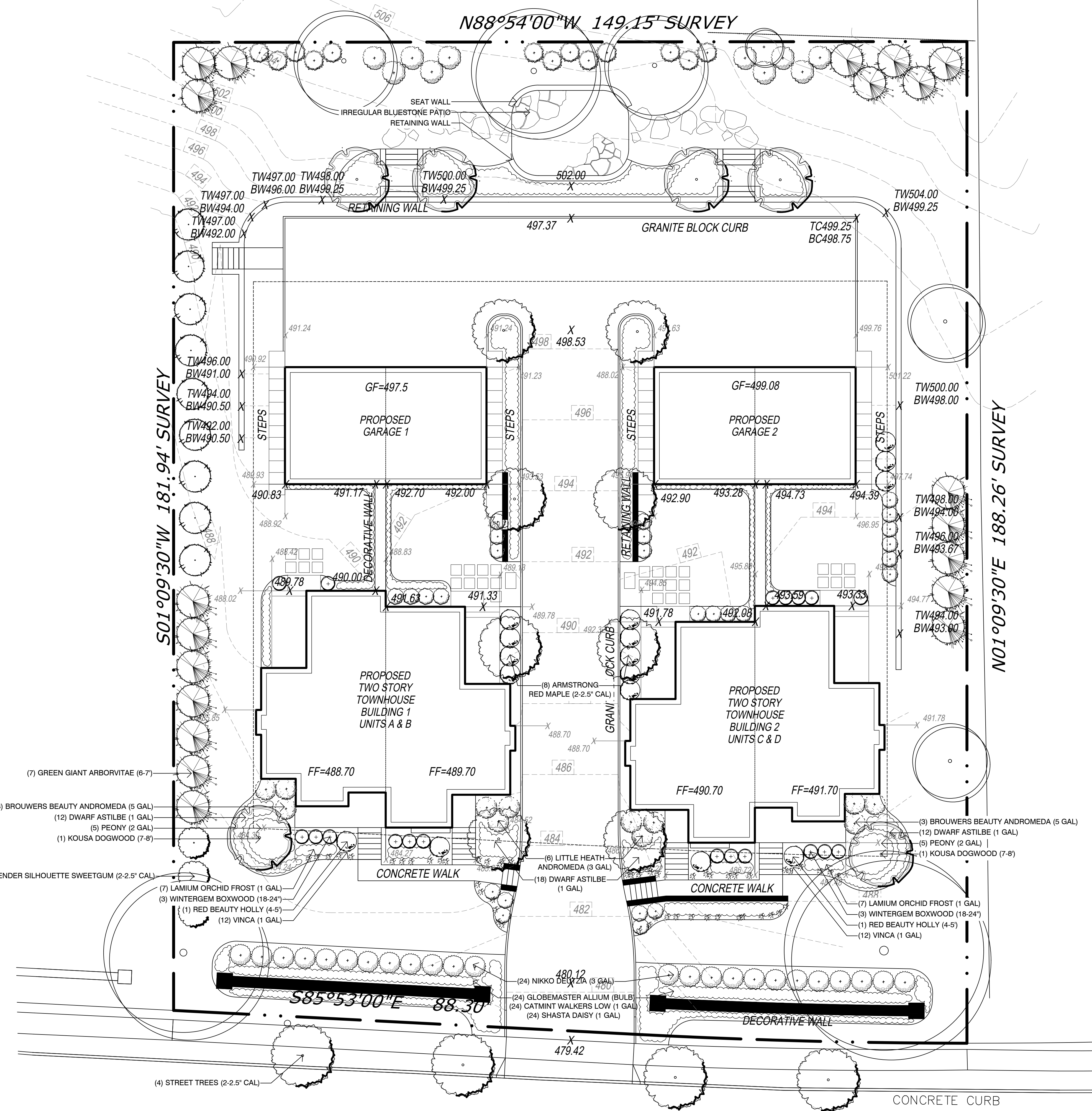
Landscape Plan Scale: 1" = 10'-0"
