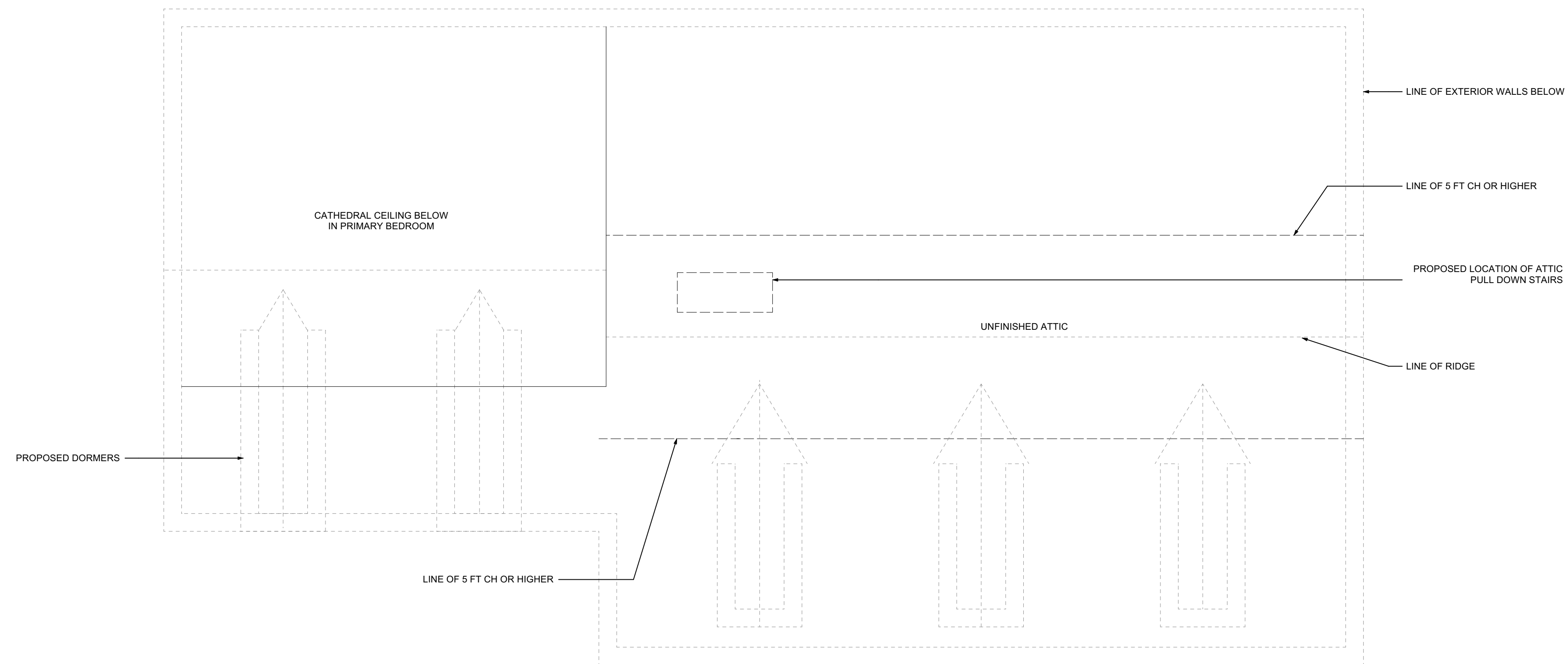
1 ATTIC PLAN Scale: 1/4" = 1'-0" UNFINISHED ATTIC AT 5 FT CH OR HIGHER: 344 SF
